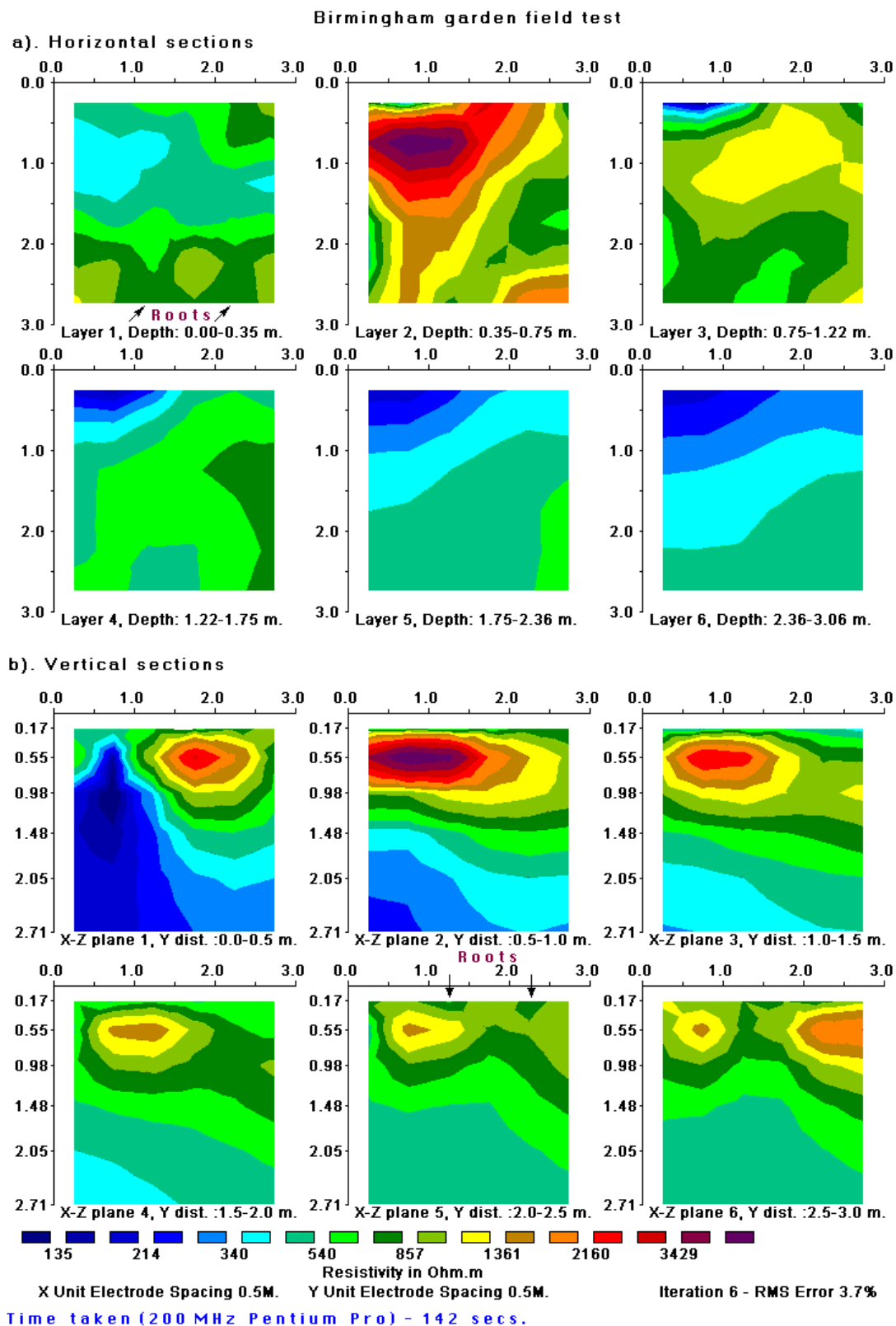
Figure 35. Horizontal and vertical cross-sections of the model obtained from the inversion of the Birmingham field survey data set. The location of observed tree roots on the ground surface are also shown.
